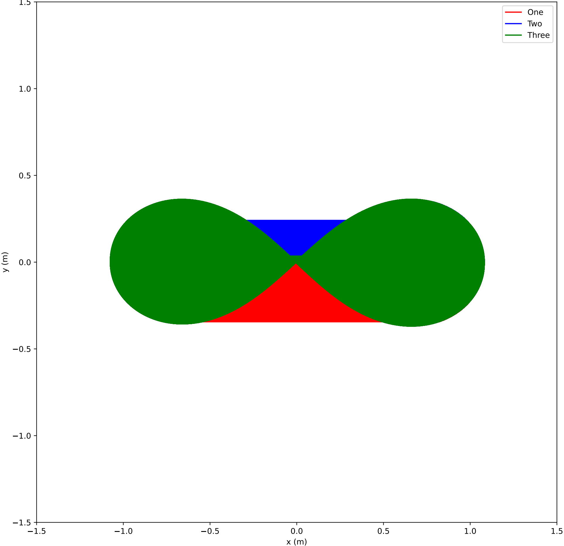
Stable (Figure-Eight) Three-Body Trajectory Integrated with the Symplectic Euler Method
